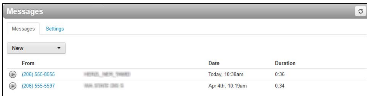
Figure 2-5. Messages Page
