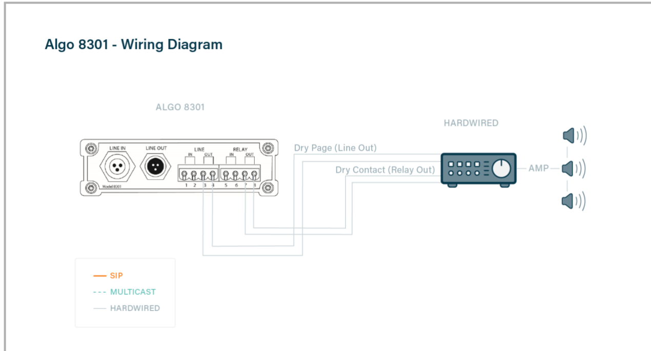
Figure 4: Use Case Wiring Diagram
