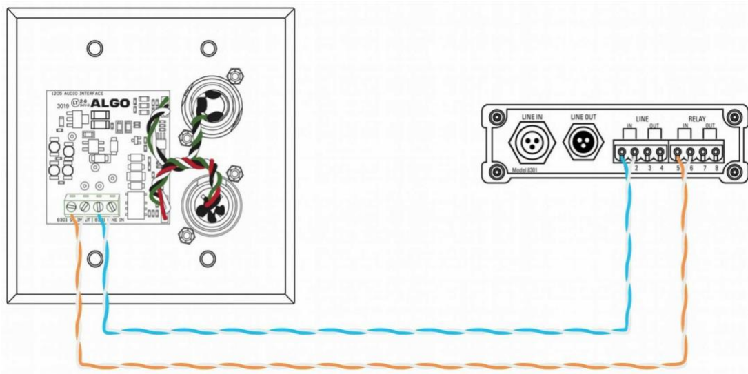
Figure 9: 1205 Audio Interface Wiring
