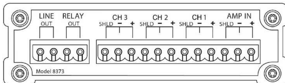
8373 Zone Paging Adapter: Back View
